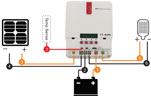
Figure 2-3 Wiring
