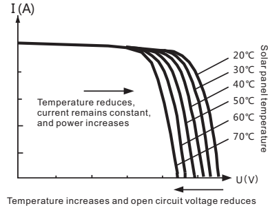
Figure 1-4 Solar Panel Output Characteristic and Temperature Relation
