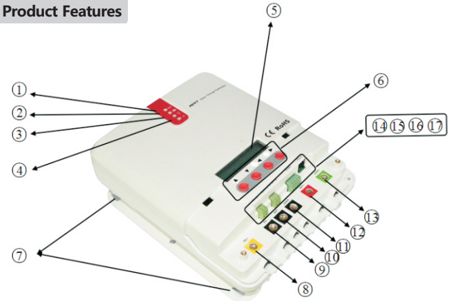
Figure 1-1 Solar Charge Controller Appearance and Interface
